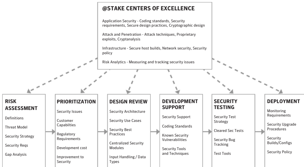
Figure 1: The Symantec @stake Secure Development Lifecycle (S@SDL)
